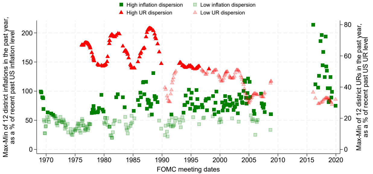
(c) Dispersion.
