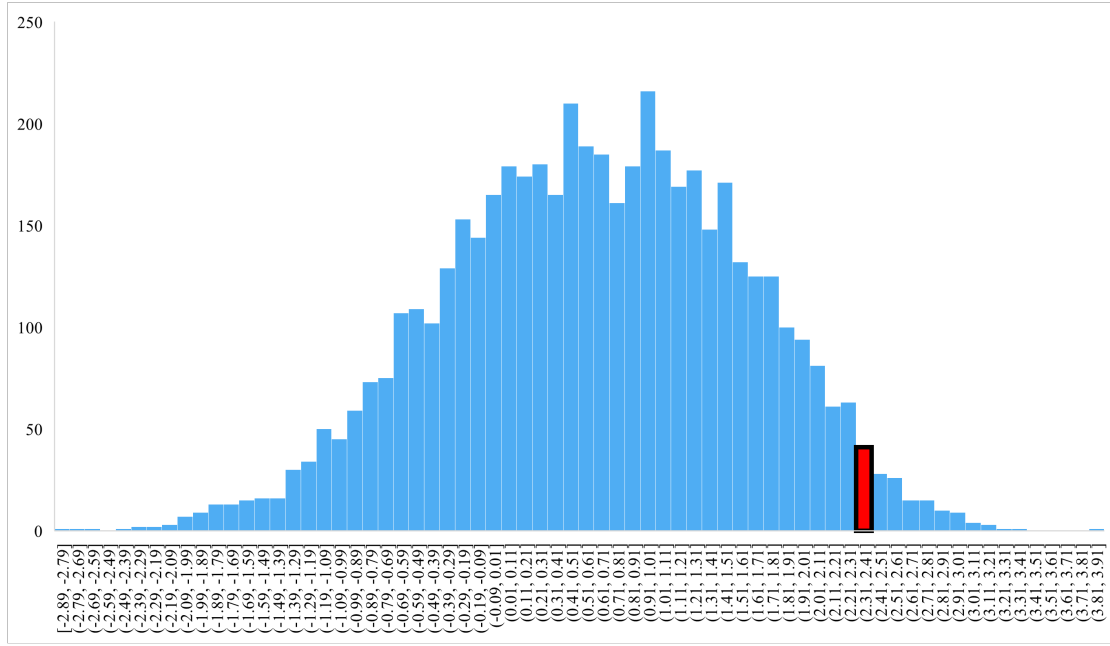
(a) Inflation
